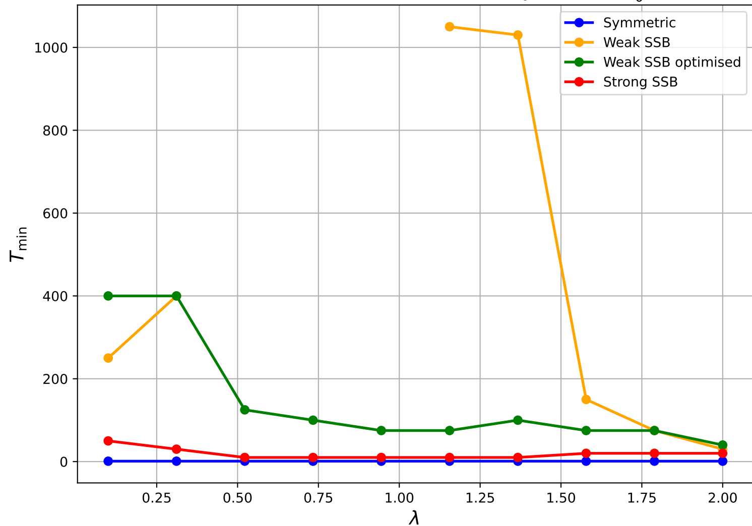
Minimum Adiabatic Time T_{\min} for Fidelity \geq 0.97 , m_0^2 = 1
